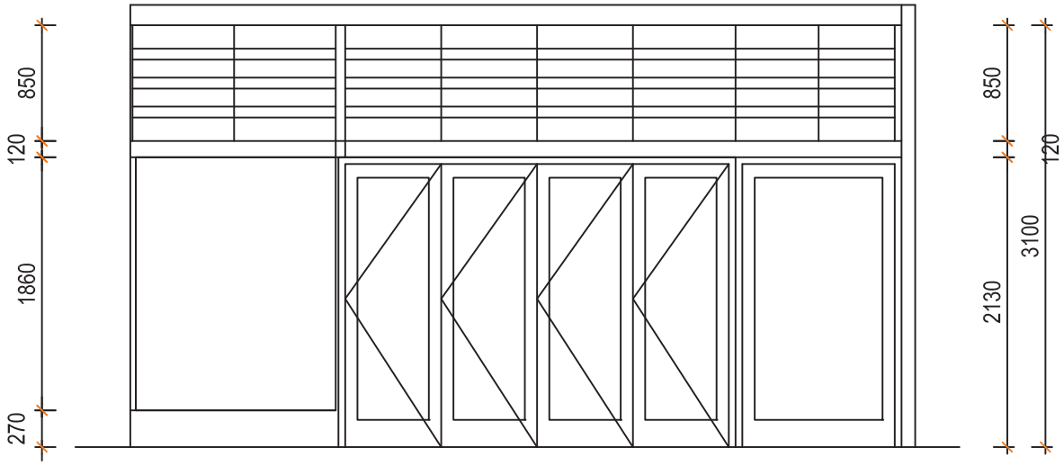
front elevation
